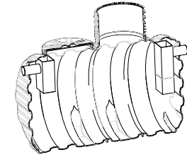
Grease sep. in 5m³ tank
