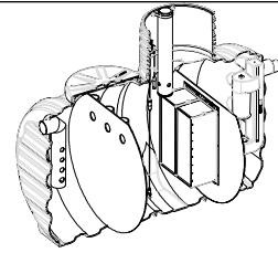
Oil sep. NS3 with sludge trap and ACD
