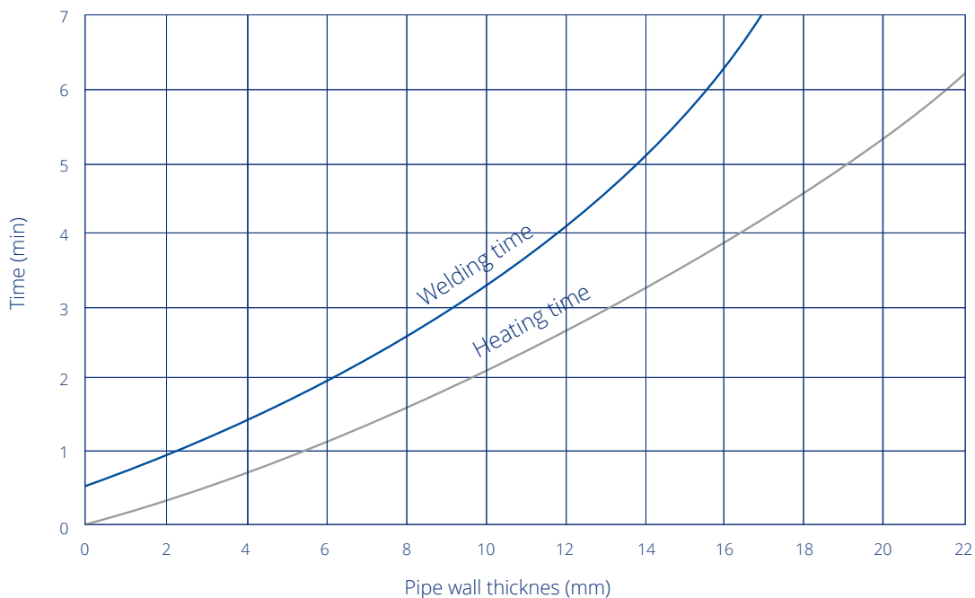
Welding diagram
