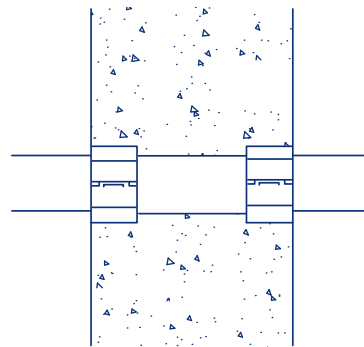
Passage through the floor — internal location
